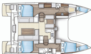
3 Cabin Layout
